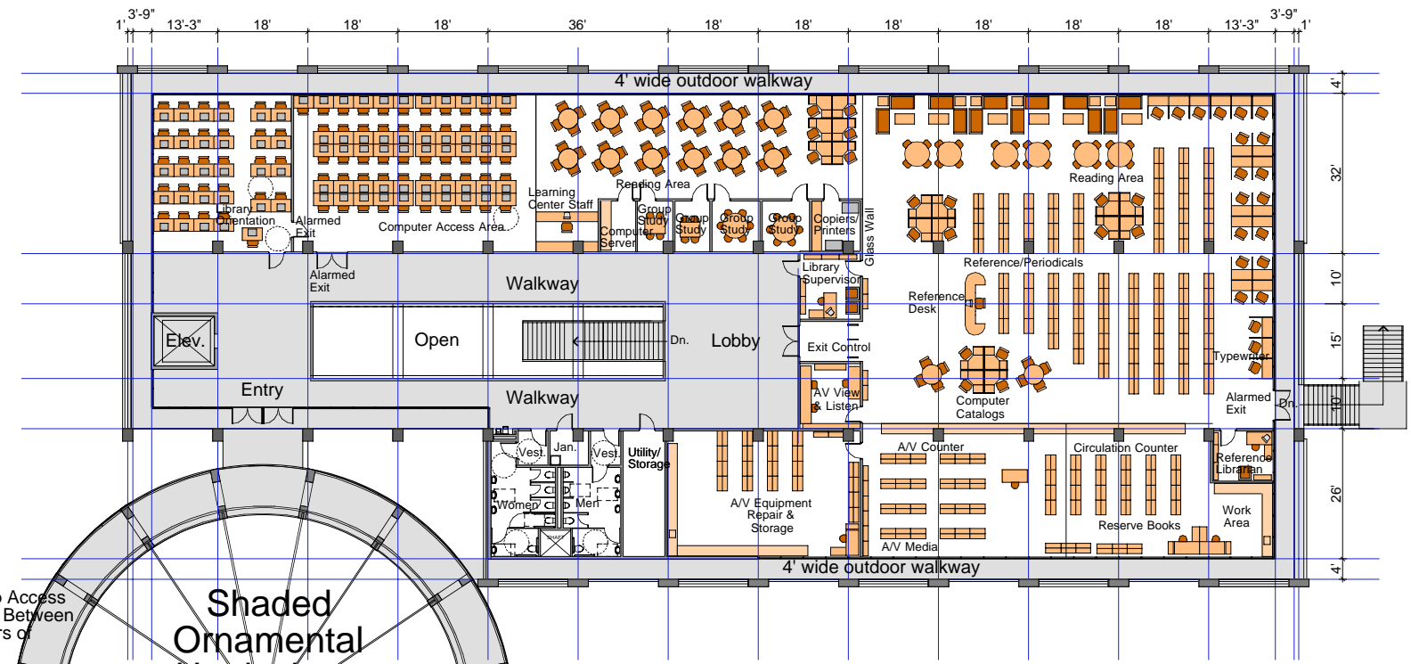
2nd Floor -- Library, AV/TV
